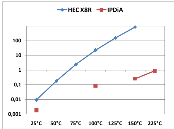
Fig.7: FIT rates calculated at 60% confidence level
