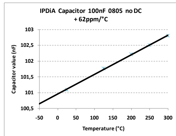
Fig.3: Capacitance dependence on temperature.
